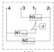
900 HOTPLATE 300x300 4000 watt
